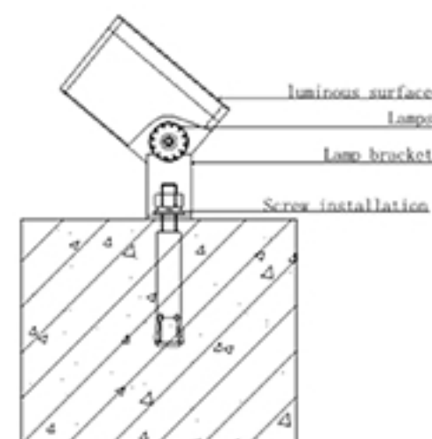
Installation Illustration
