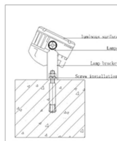
Installation Illustration
