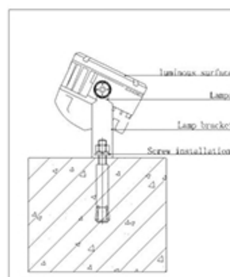
Installation Illustration
