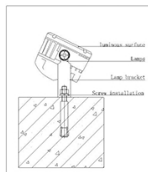
Installation Illustration
