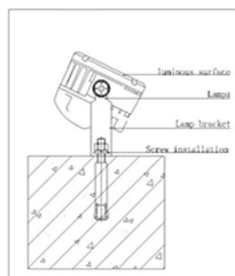
Installation Illustration
