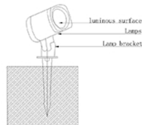
Installation Illustration
