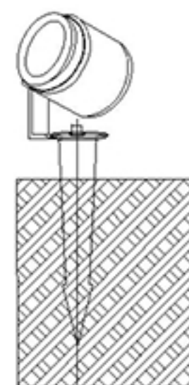
Installation Illustration
