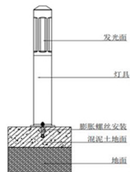
Installation Illustration
