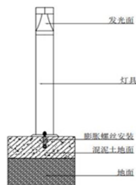
Installation Illustration
