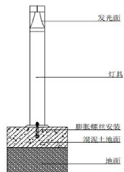
Installation Illustration
